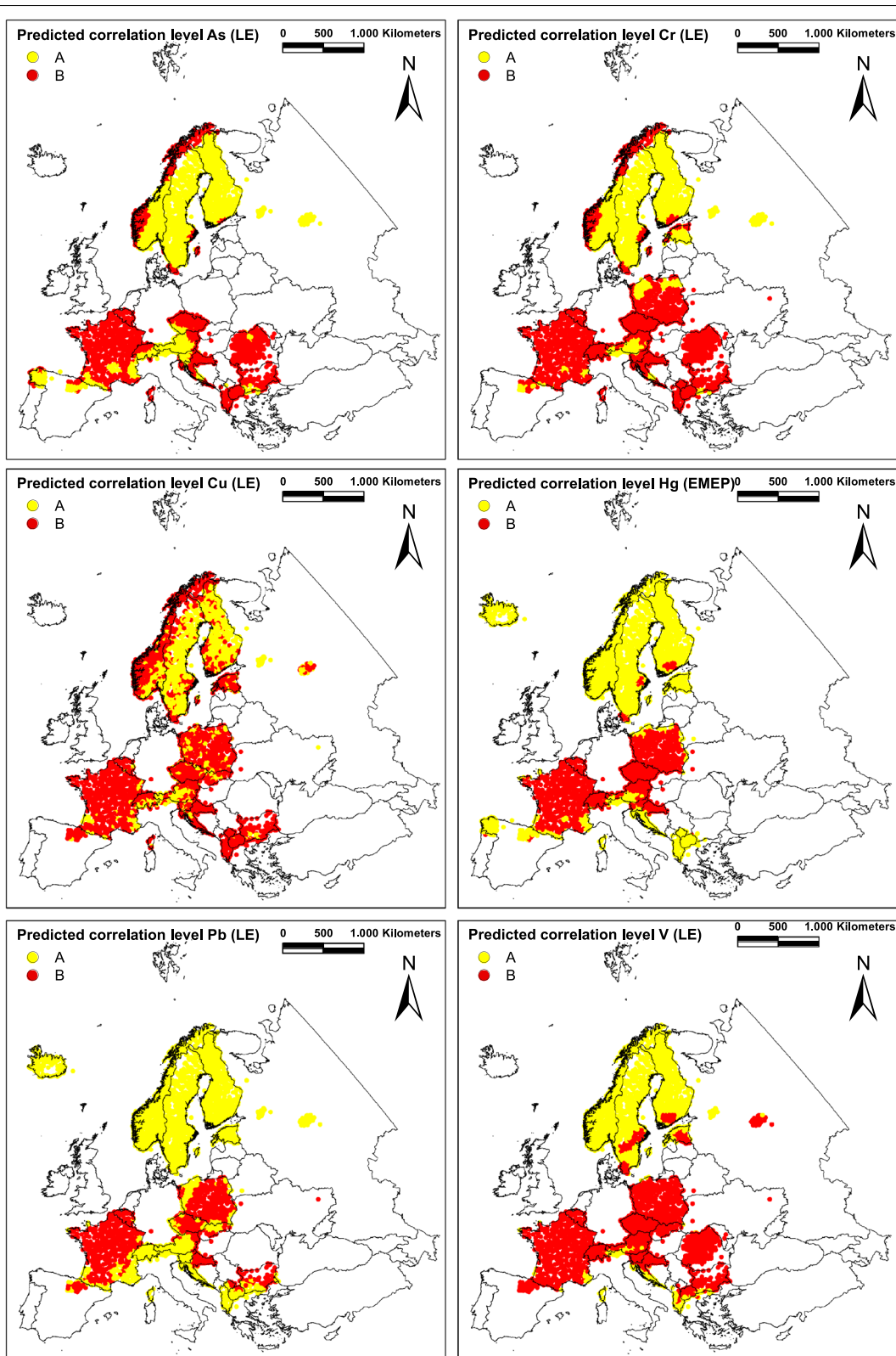
Fig. 5 Predicted correlation patterns for As, Cr, Cu, Hg, Pb, and V (moss; EMEP/LE) at site level as classified according to their surrounding land use with above element-specific average (= A) or below-average (= B) correlations (cf. Table 2)
